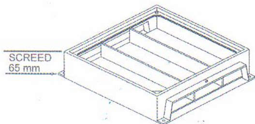
2-WAY JUNCTION BOX CODE: 2WJB-7
