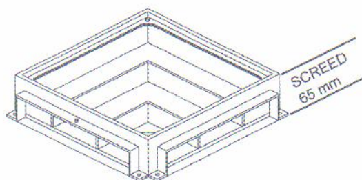
90° ANGLE JUNCTION BOX CODE: 90JB-4
